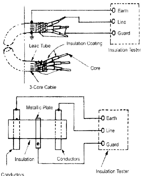
Fig. 4 Typical Guard Terminal Application
