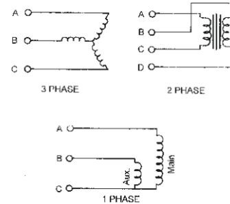
Fig. 1 Common A.C. motor and generator type
